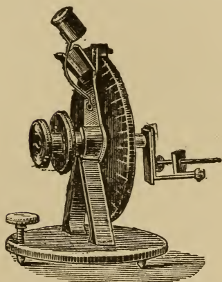
Fig. 88. WOLLASTON'S REFLECTING ANGLE MEASURER FOR CRYSTALS.
